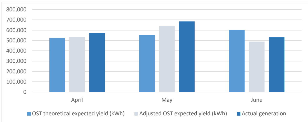
Figure 1: Monthly generation
