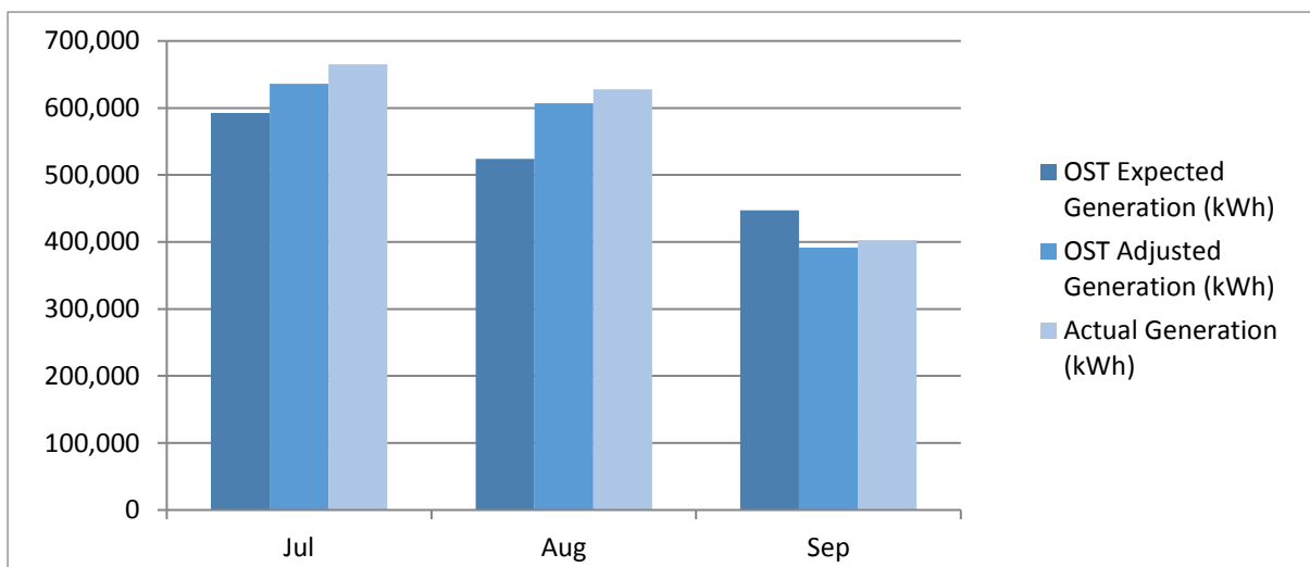
Figure 1: Monthly generation
