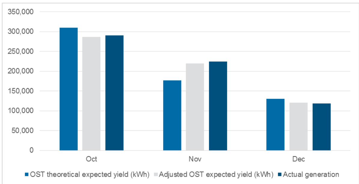
Figure 1: Monthly generation
